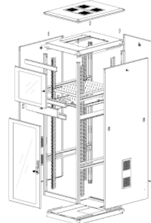
EXPLODED VIEW
